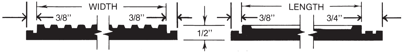
Typical Locklip Safety Mat Cross Section Detail
