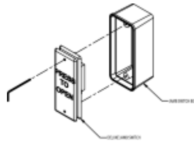
Jamb Box Mounting (Surface Mount Only)
