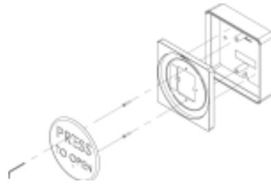
Universal Box Mounting for 6" & 4" Switches (Surface Mount)
