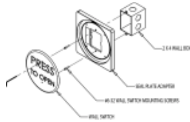
2 x 4 (Single-Gang) Electrical Box Mounting for 6" & 4-1/2" Switches
